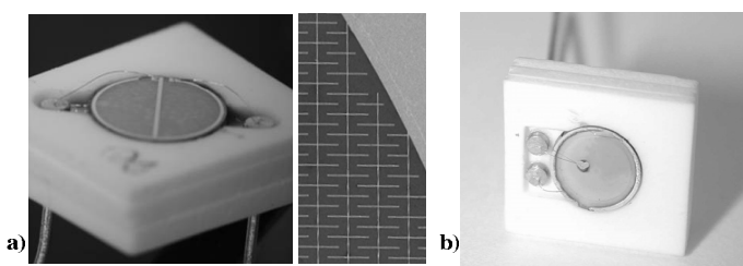
Fig. 6. Photograph of the diamond photodetectors a) MSM and detail of the Ti/Pt/Au contact structures; b) the PIN photodiode.
